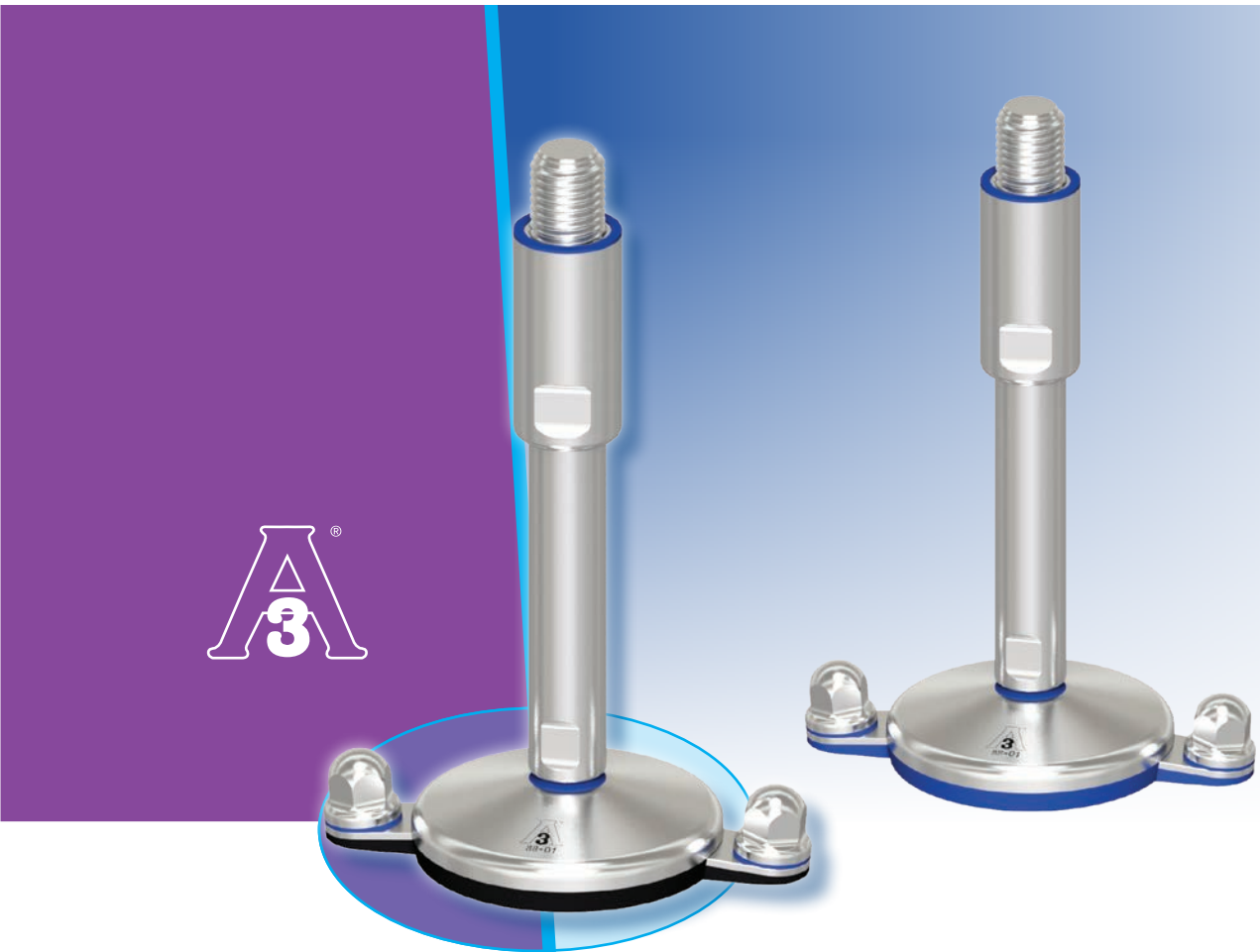
3-A TEKNO-HYGIENIC FOOT WITH Ø120 STAINLESS STEEL VULCANIZED BASE, DOUBLE FIXING
